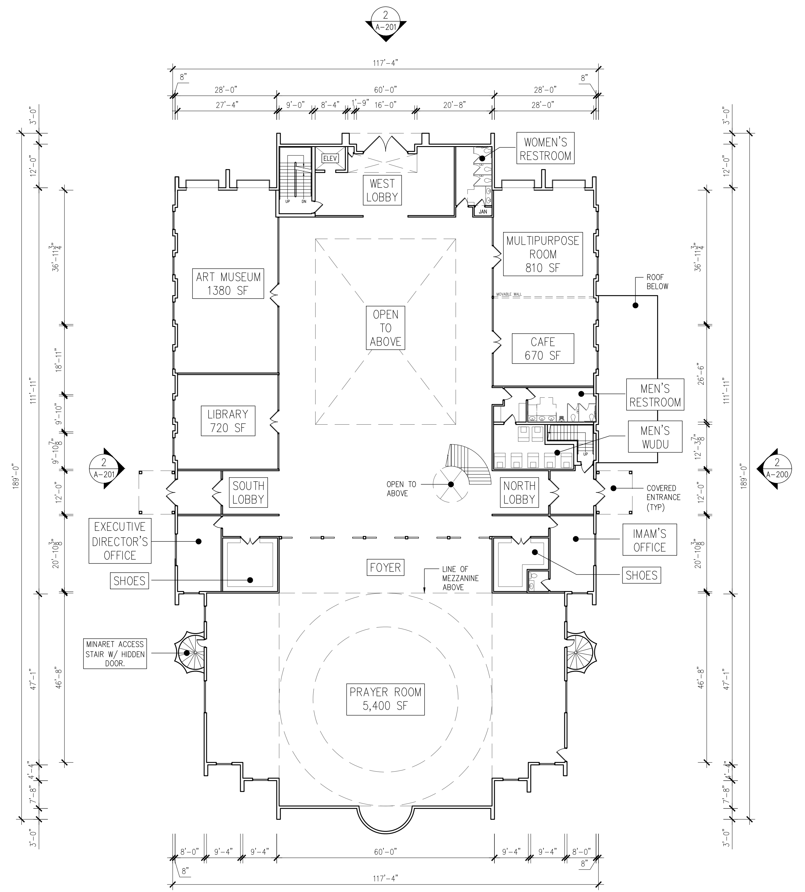
2 FIRST FLOOR SCALE: 1/16" = 1'-0"
