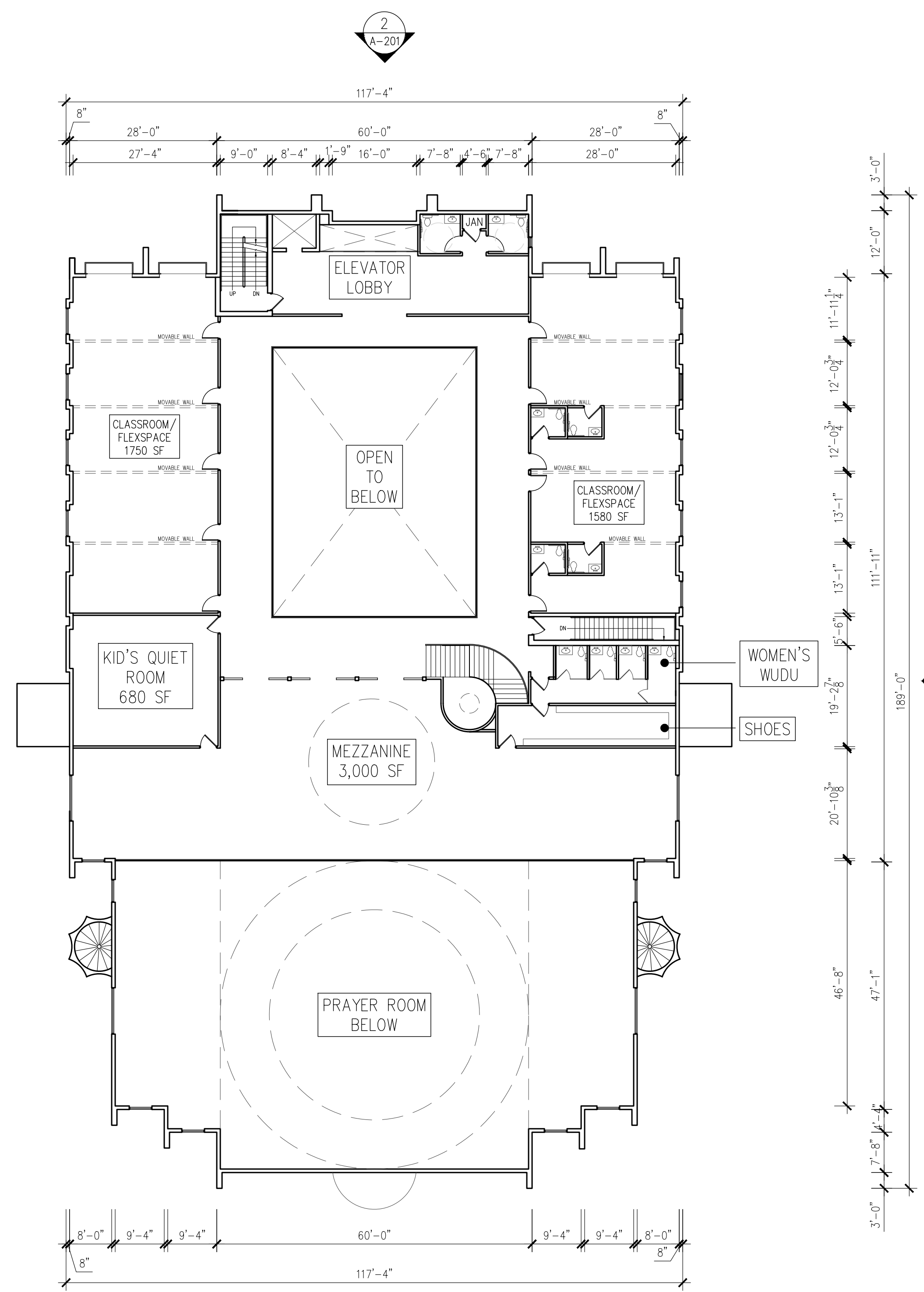
1 SECOND FLOOR SCALE: 1/16" = 1'-0"
