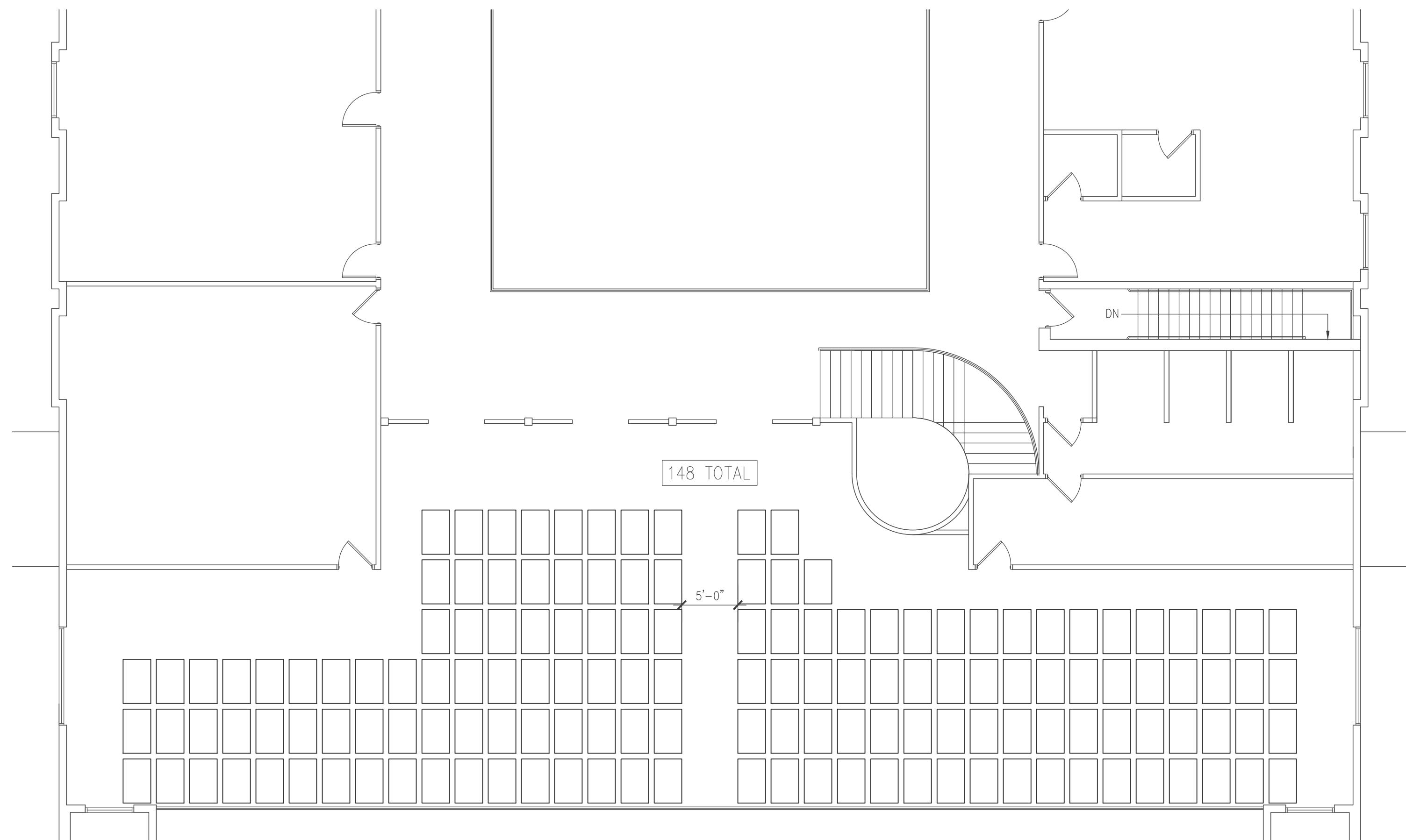
2 ENLARGED MEZZANINE SEATING PLAN A-102 SCALE: 1/8" = 1'-0"
