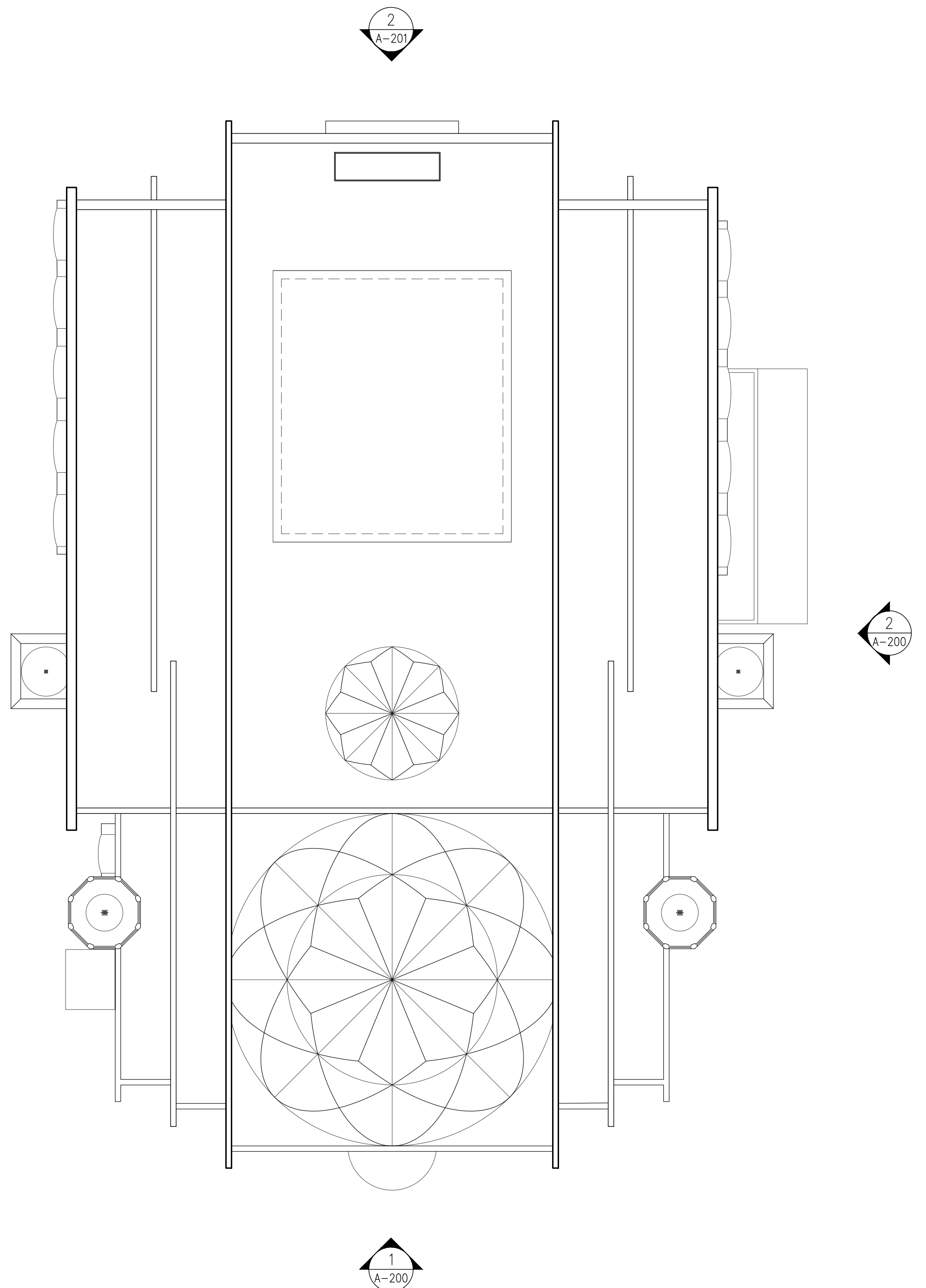
1 ROOF PLAN SCALE: 1/16" = 1'-0"
